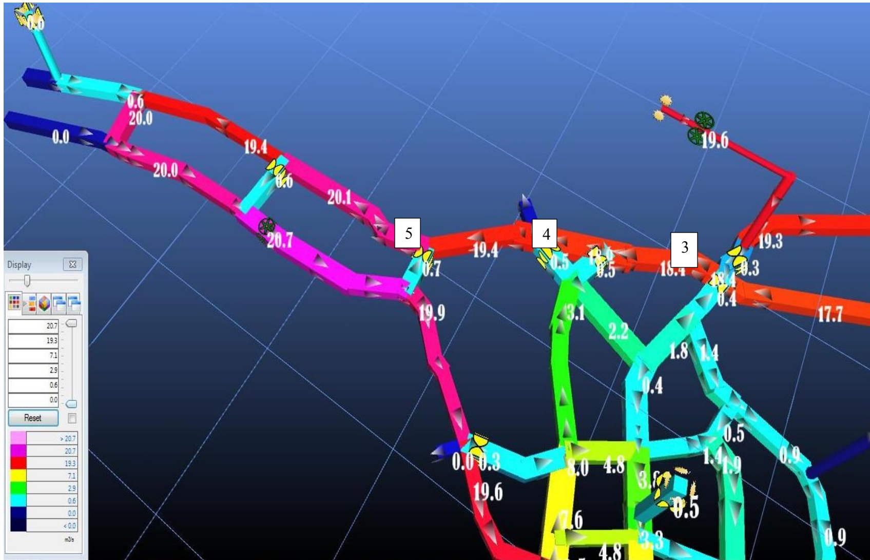
Figure 5.13 Main fan and west booster fan at blade set 5 simulated results
